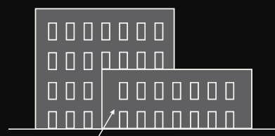
VENTILATED FACADE
